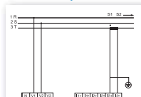
Unbalanced 3-phase, 3 wires - 2 CTs
