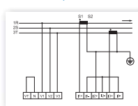
Unbalanced 3-phase, 3 wires - 2 CTs
