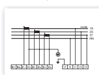
Example of connection to VT
