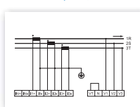
Unbalanced 3-phase, 3 wires - 3 CTs
